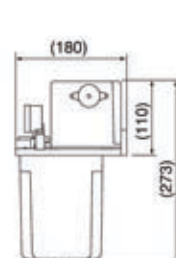
DYET-A1-4L Aluminum alloy tank
